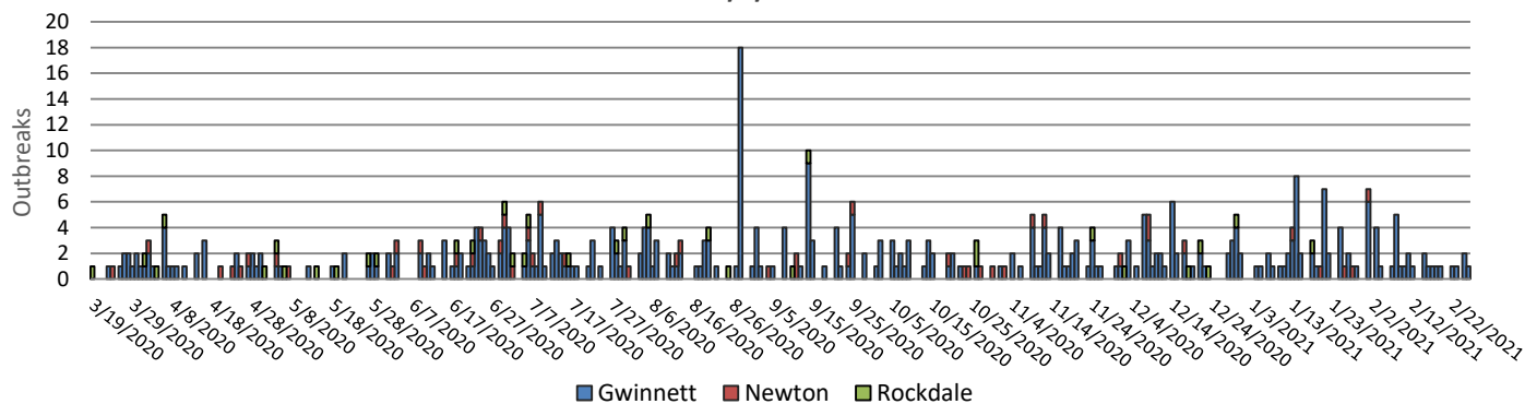
Number of Outbreaks Per County Over Time, Gwinnett, Newton and Rockdale Counties, as of 3/1/2021
