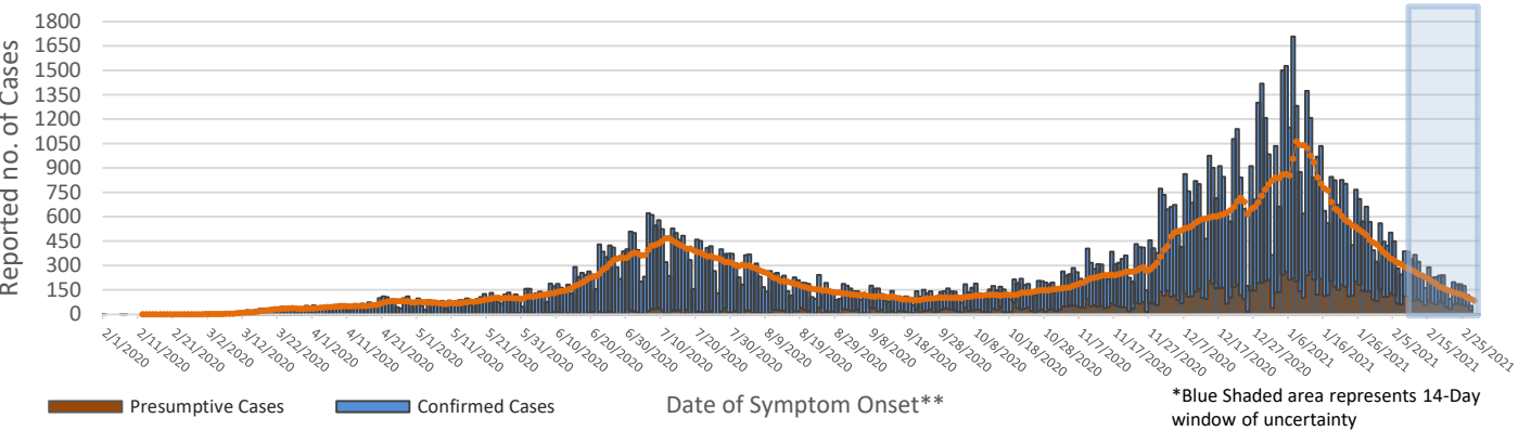
Reported COVID-19 Cases in residents of Gwinnett, Newton, and Rockdale Counties, as of 3/1/2021 †
